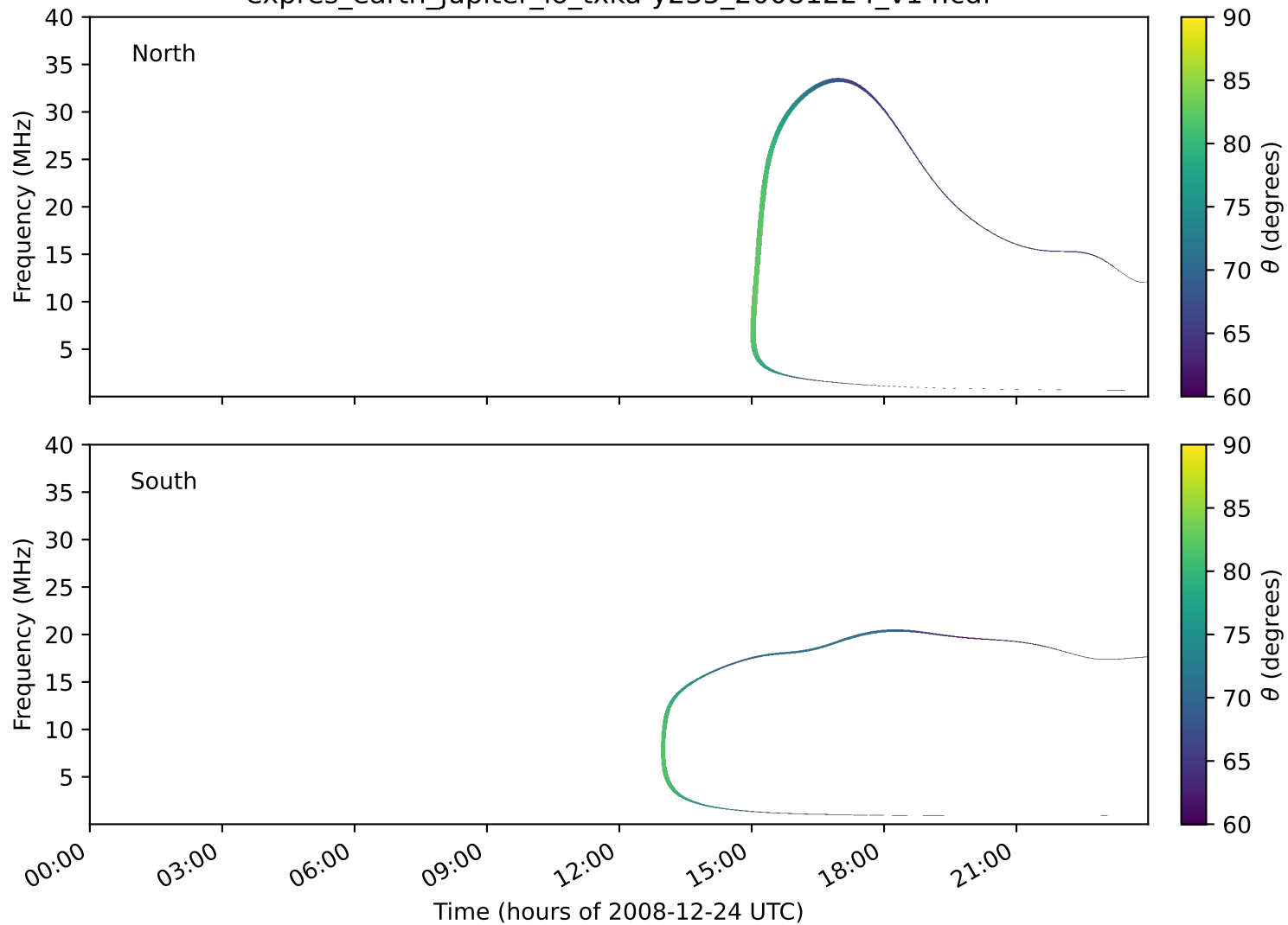
expres_earth_jupiter_io_txka-y235_20081224_v14.cdf
