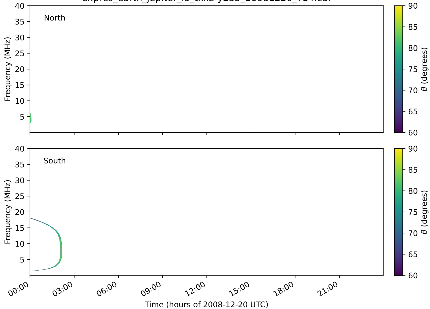
expres_earth_jupiter_io_txka-y235_20081220_v14.cdf
