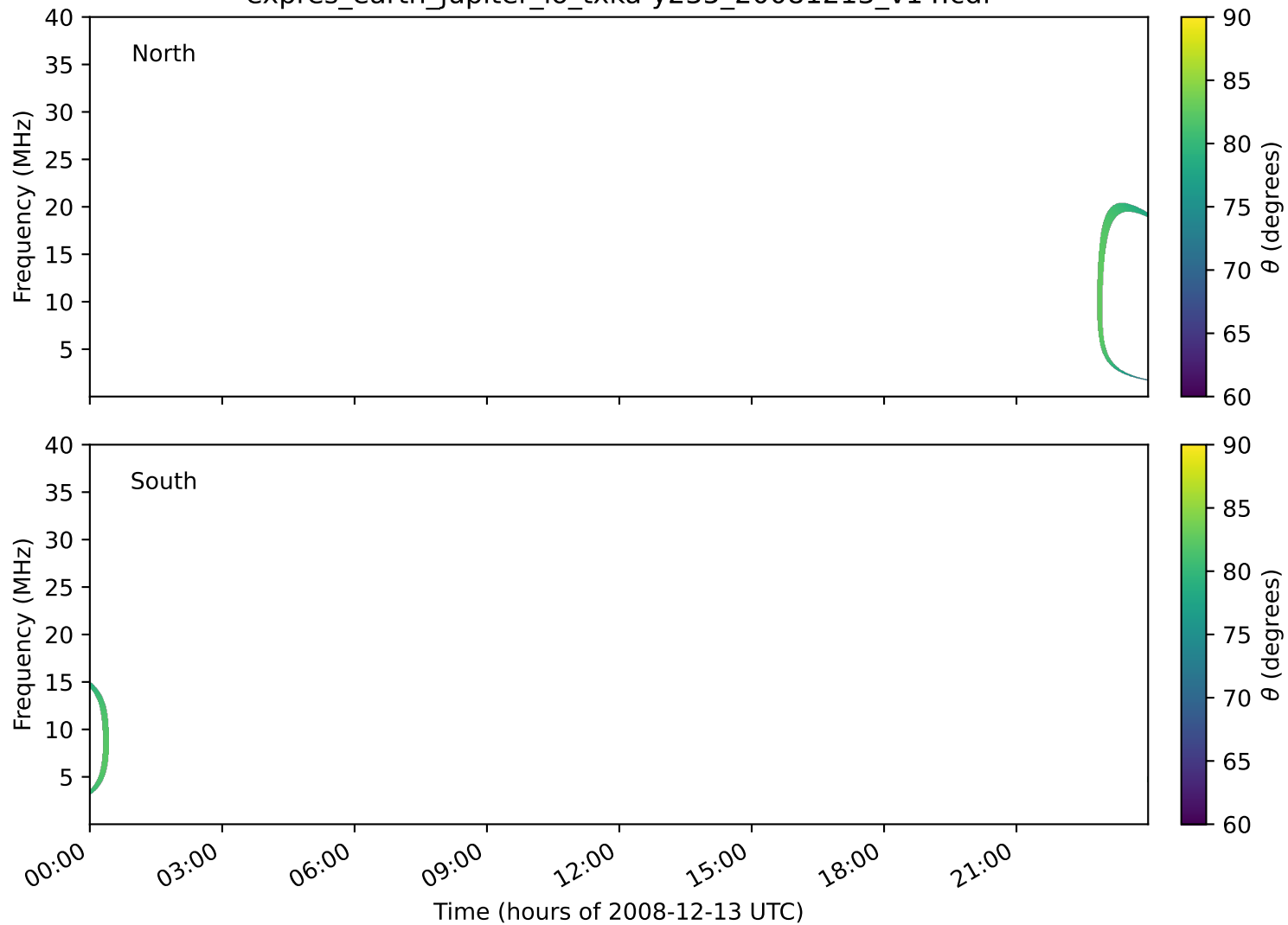
expres_earth_jupiter_io_txka-y235_20081213_v14.cdf
