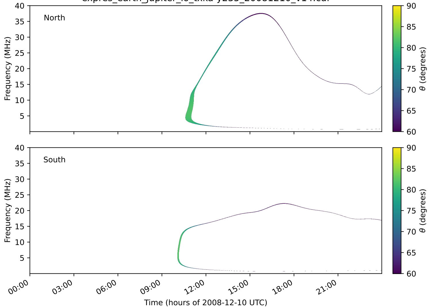
expres_earth_jupiter_io_txka-y235_20081210_v14.cdf
