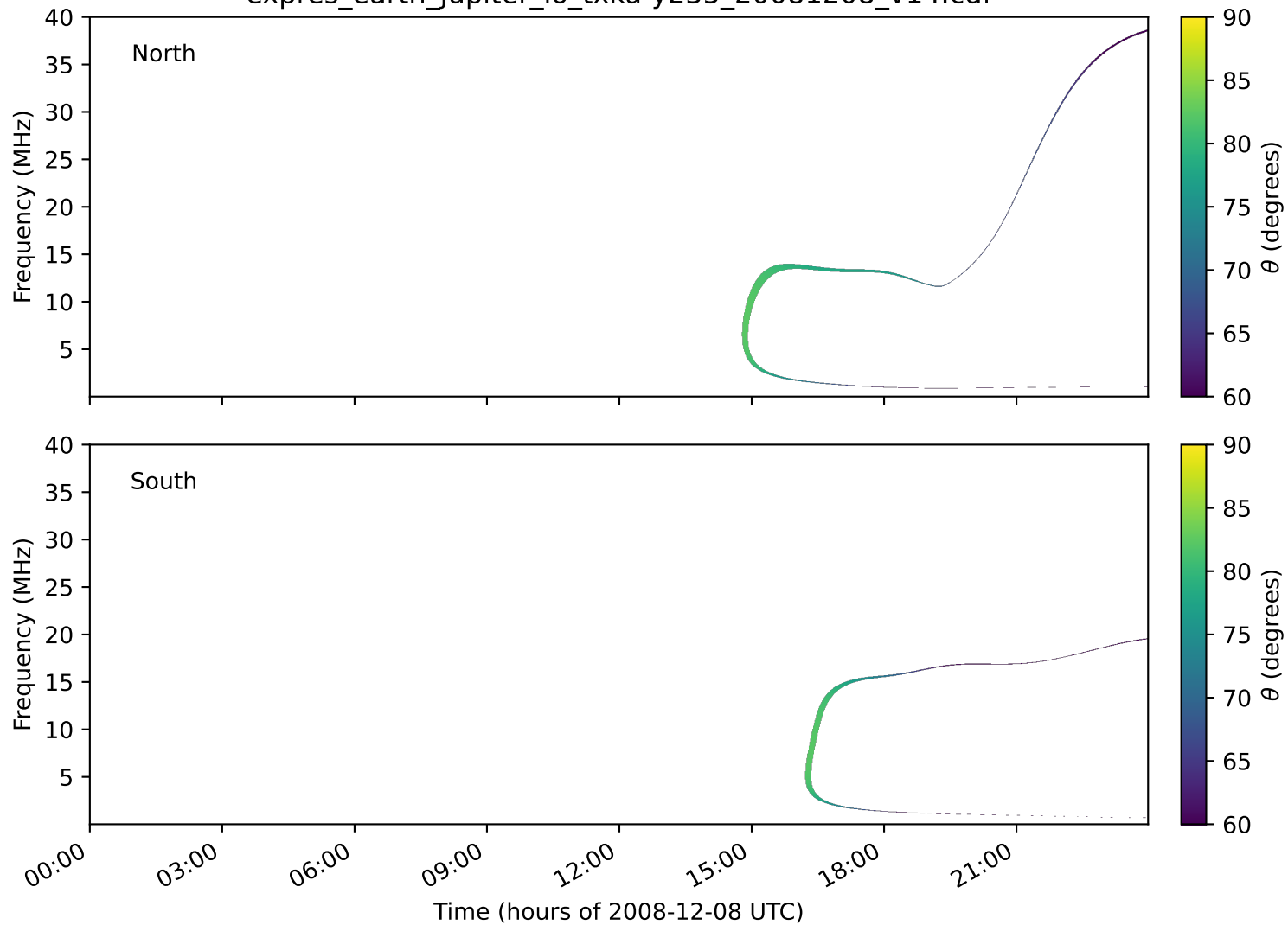
expres_earth_jupiter_io_txka-y235_20081208_v14.cdf
