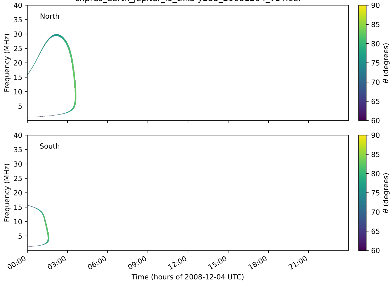
expres_earth_jupiter_io_txka-y235_20081204_v14.cdf
