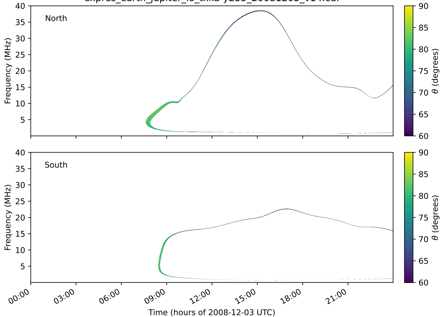
expres_earth_jupiter_io_txka-y235_20081203_v14.cdf
