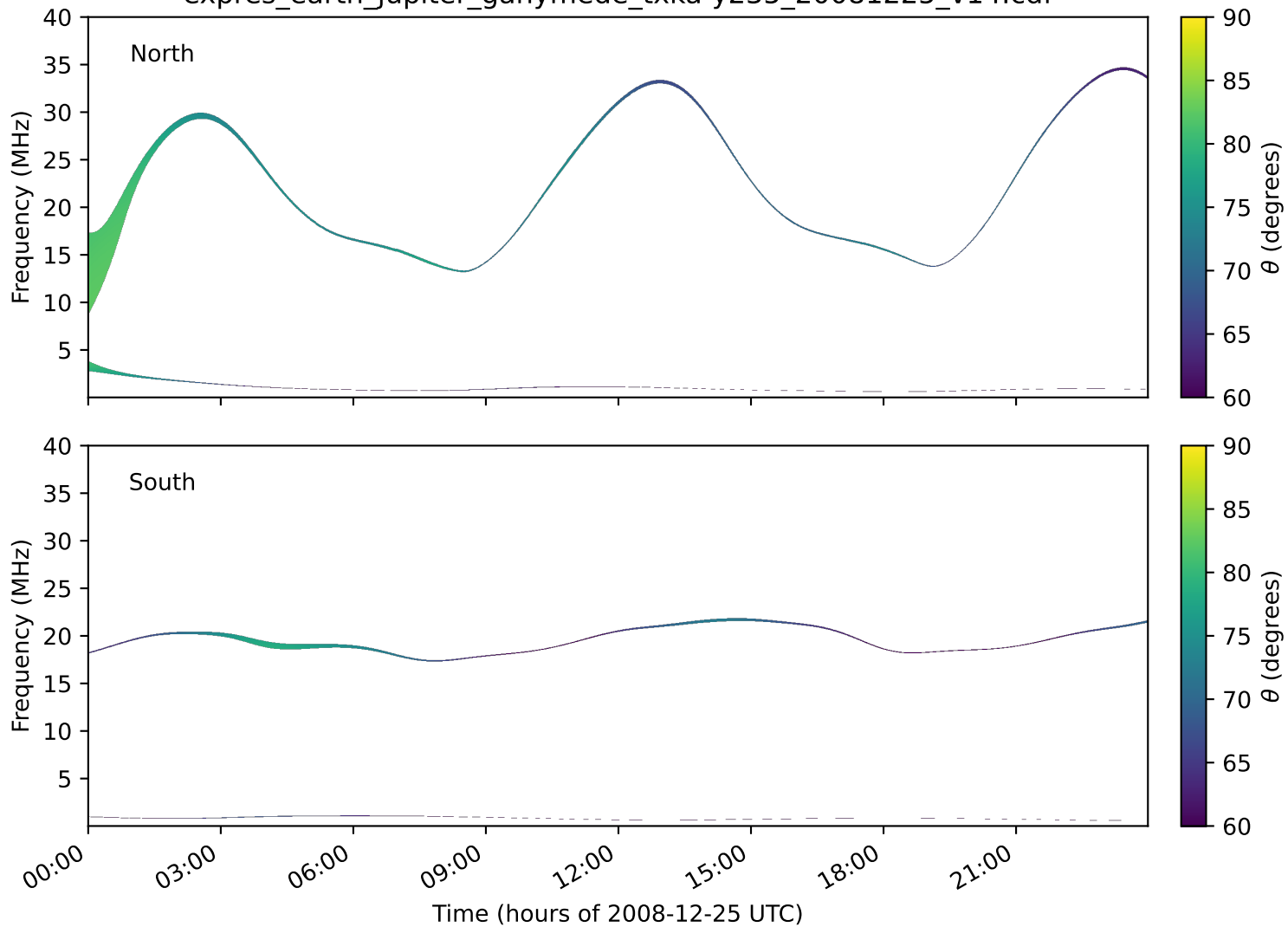
expres_earth_jupiter_ganymede_txka-y235_20081225_v14.cdf
