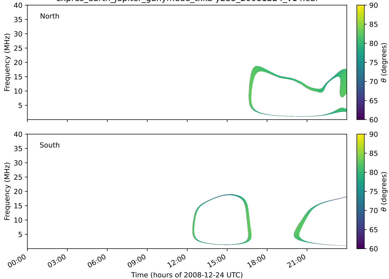
expres_earth_jupiter_ganymede_txka-y235_20081224_v14.cdf
