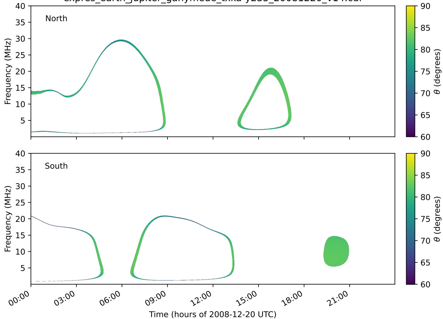
expres_earth_jupiter_ganymede_txka-y235_20081220_v14.cdf
