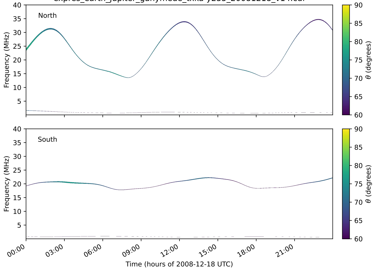
expres_earth_jupiter_ganymede_txka-y235_20081218_v14.cdf
