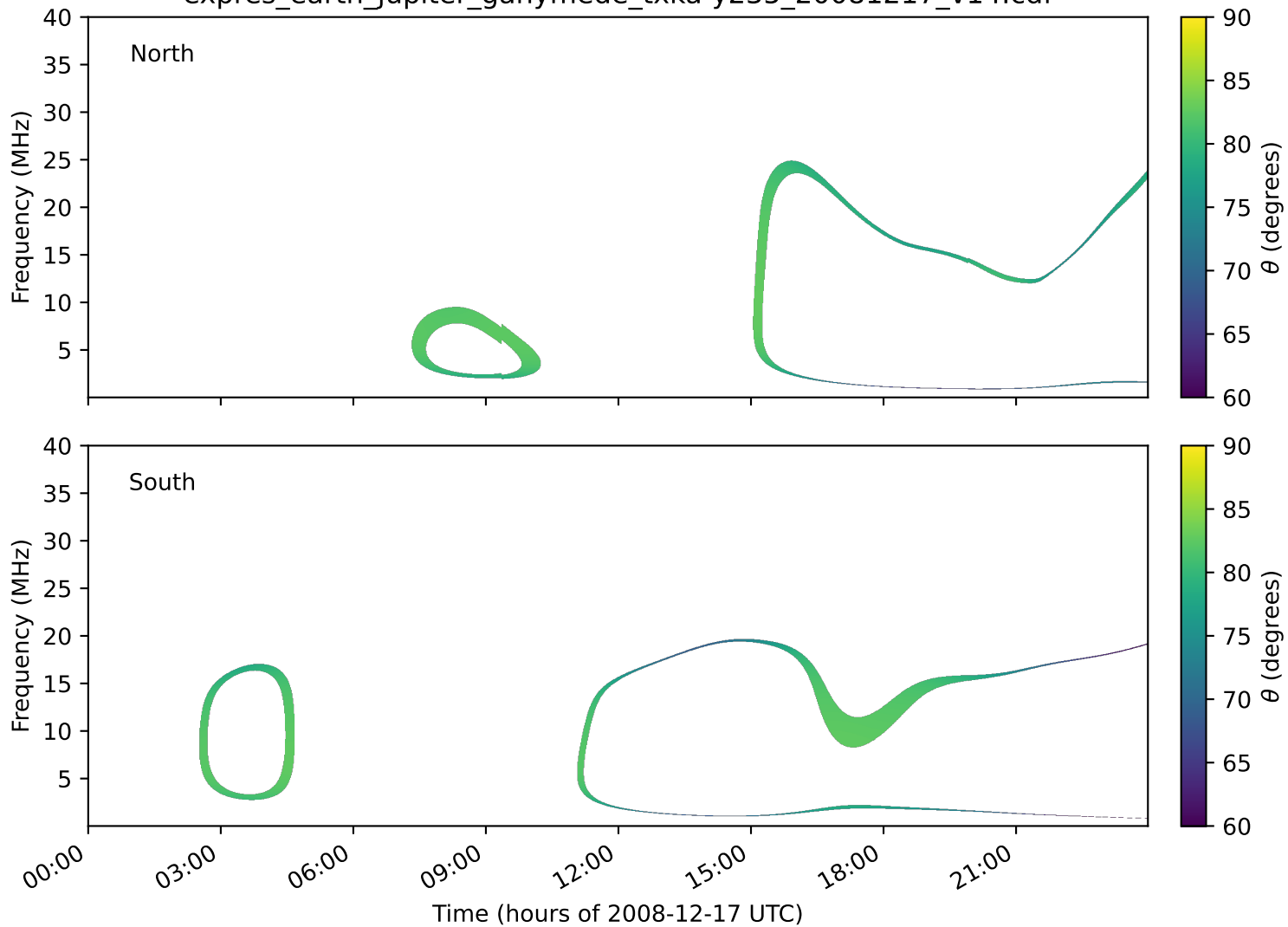
expres_earth_jupiter_ganymede_txka-y235_20081217_v14.cdf
