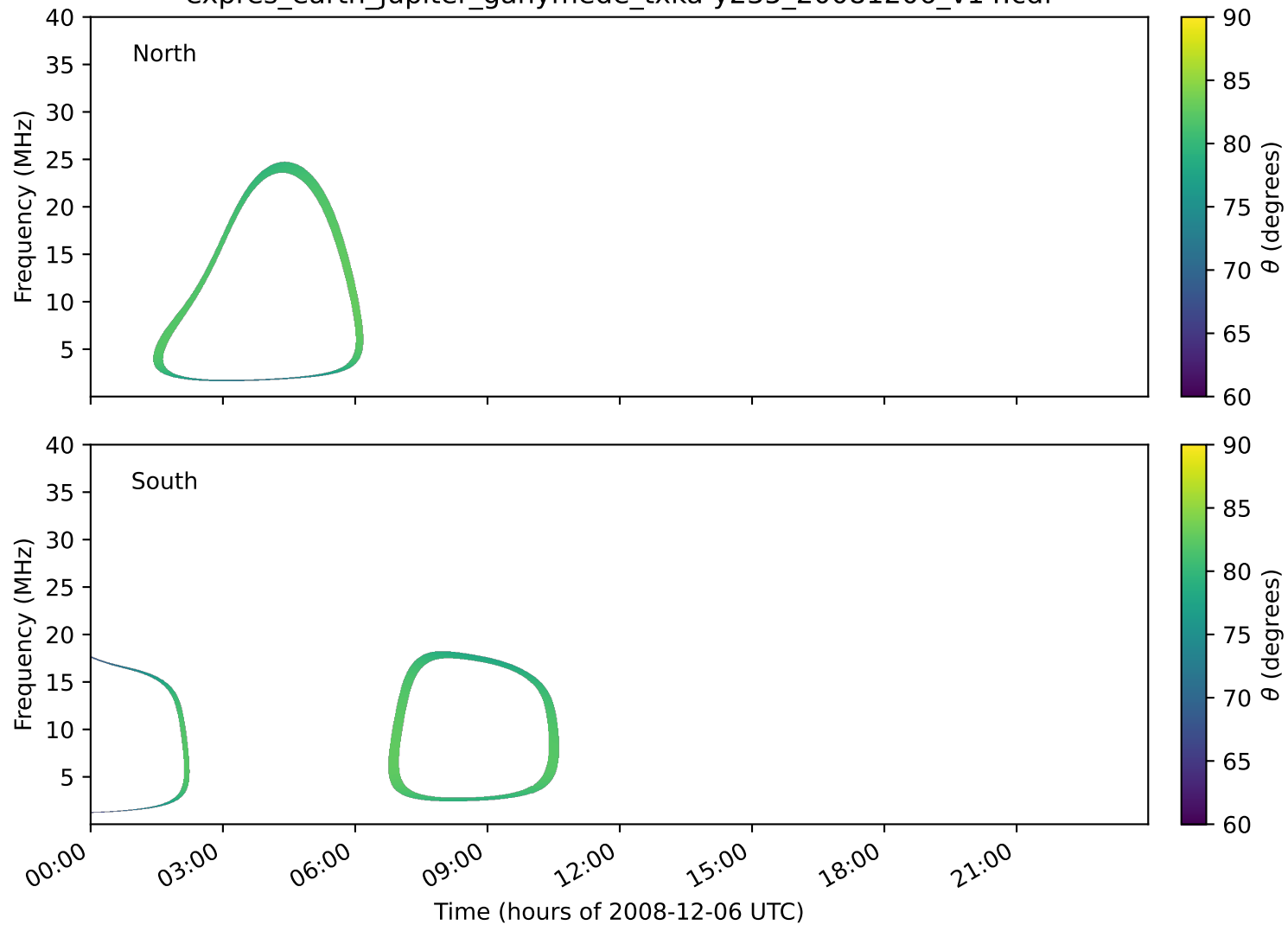
expres_earth_jupiter_ganymede_txka-y235_20081206_v14.cdf
