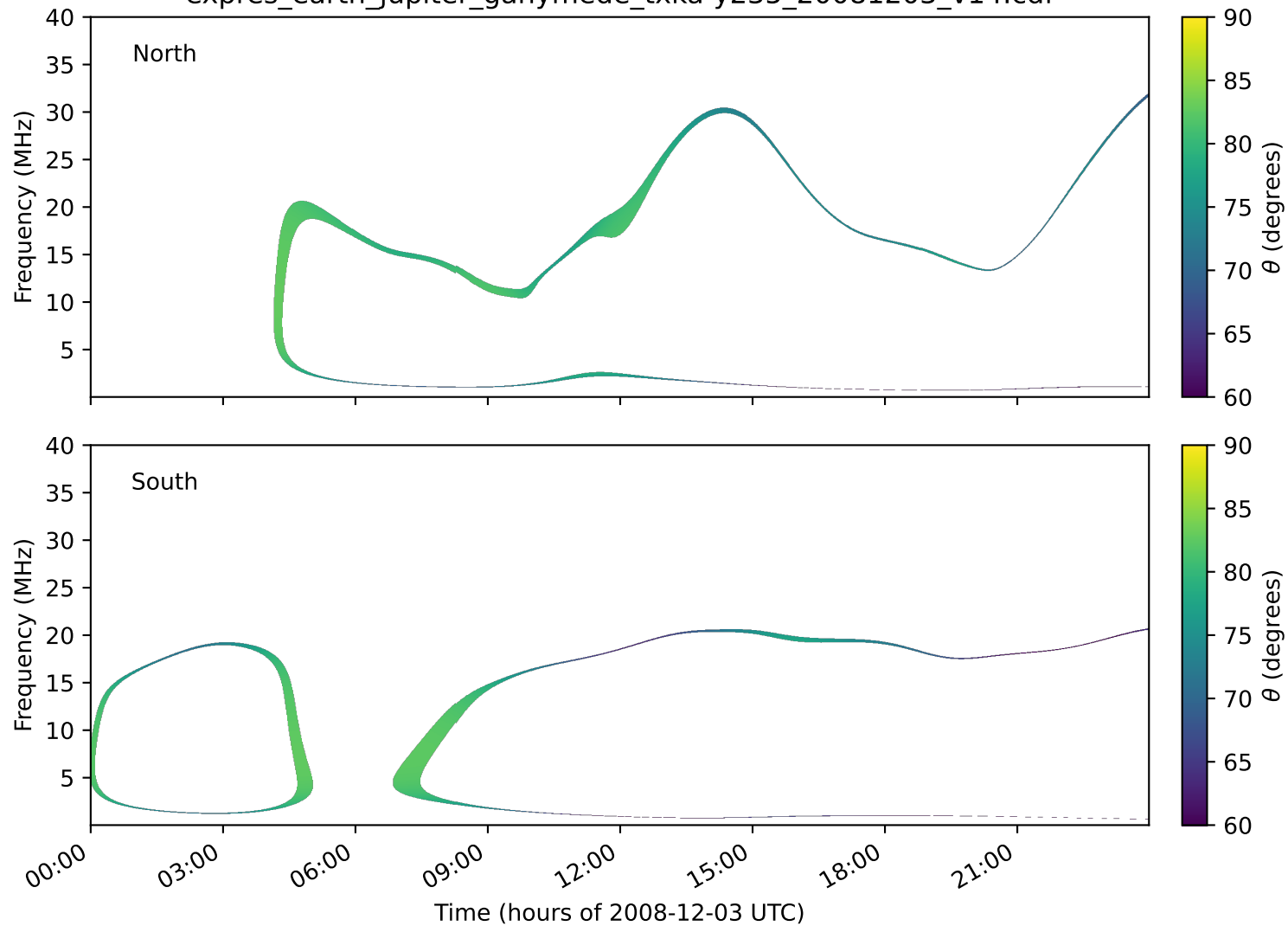
expres_earth_jupiter_ganymede_txka-y235_20081203_v14.cdf
