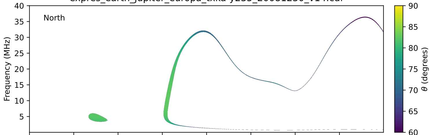
expres_earth_jupiter_europa_txka-y235_20081230_v14.cdf
