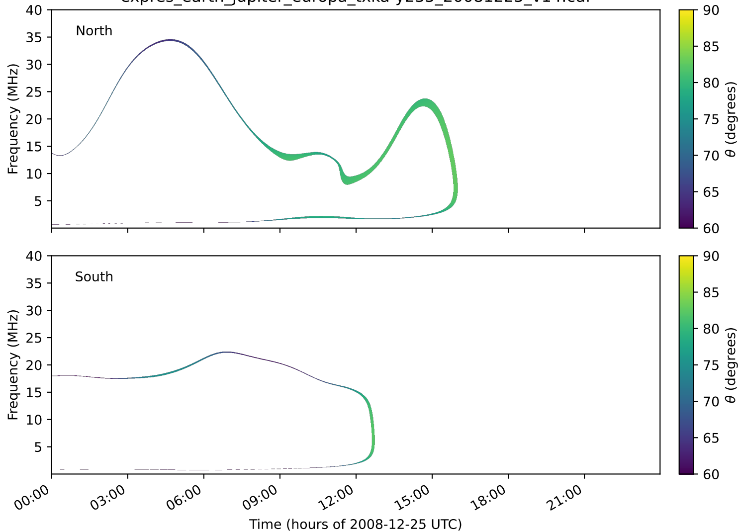
expres_earth_jupiter_europa_txka-y235_20081225_v14.cdf
