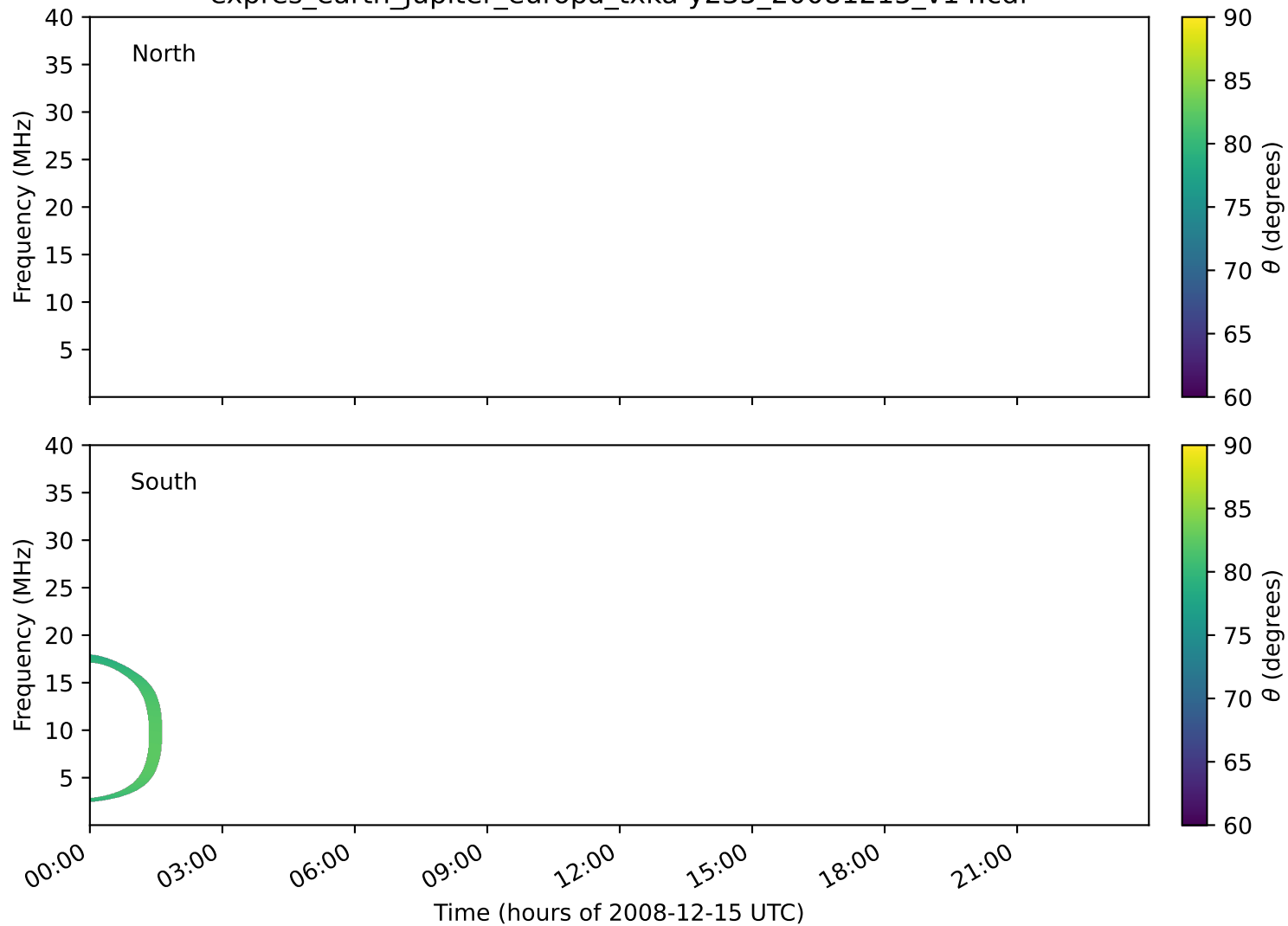
expres_earth_jupiter_europa_txka-y235_20081215_v14.cdf
