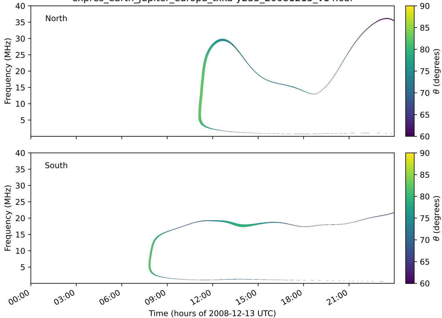
expres_earth_jupiter_europa_txka-y235_20081213_v14.cdf
