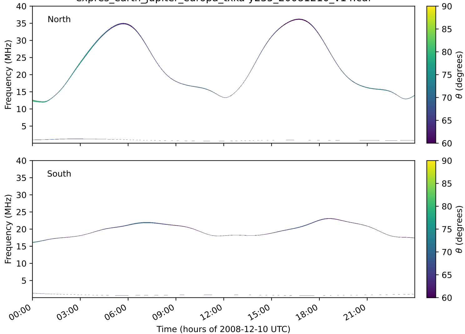
expres_earth_jupiter_europa_txka-y235_20081210_v14.cdf
