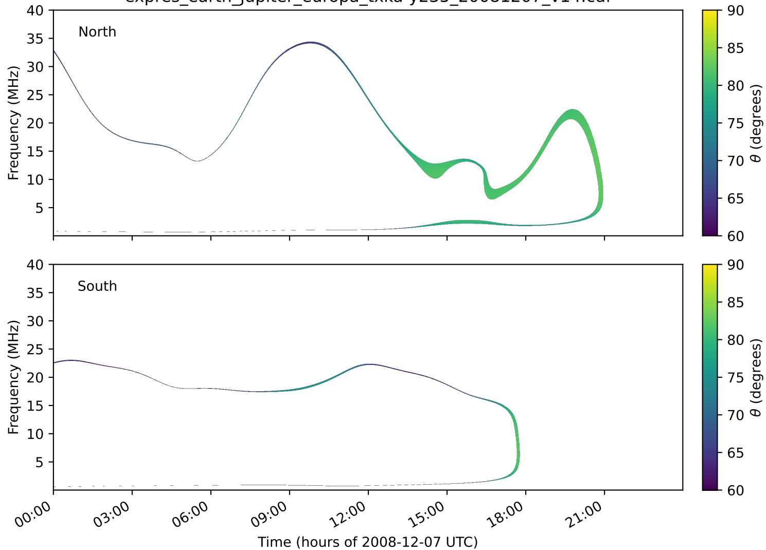
expres_earth_jupiter_europa_txka-y235_20081207_v14.cdf
