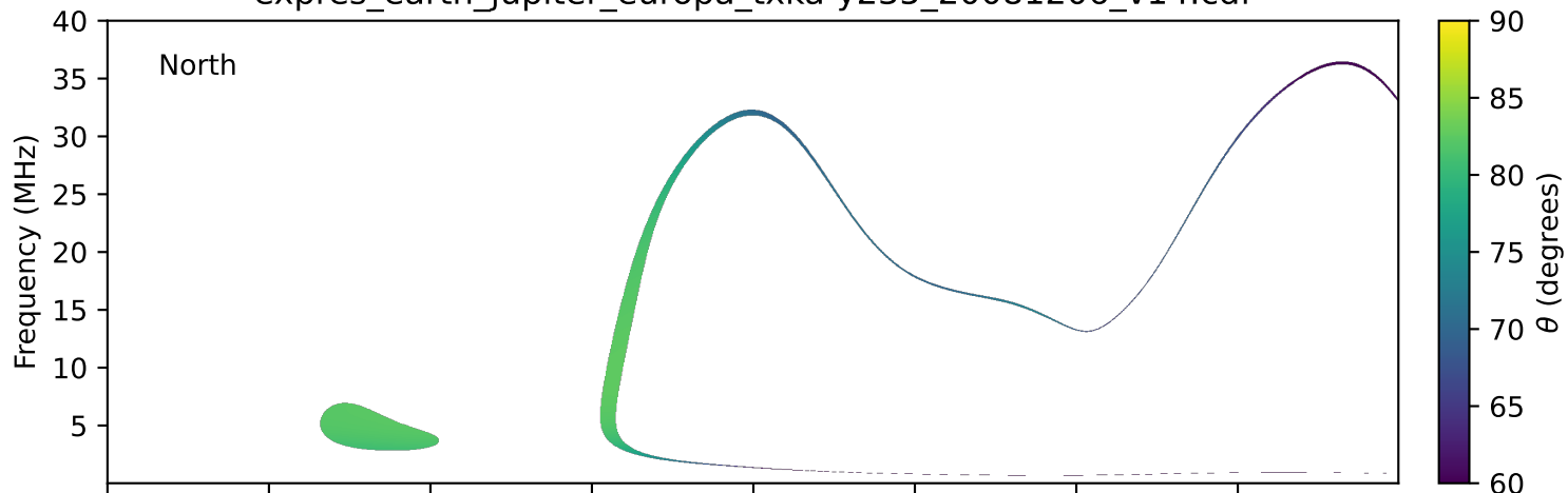
expres_earth_jupiter_europa_txka-y235_20081206_v14.cdf
