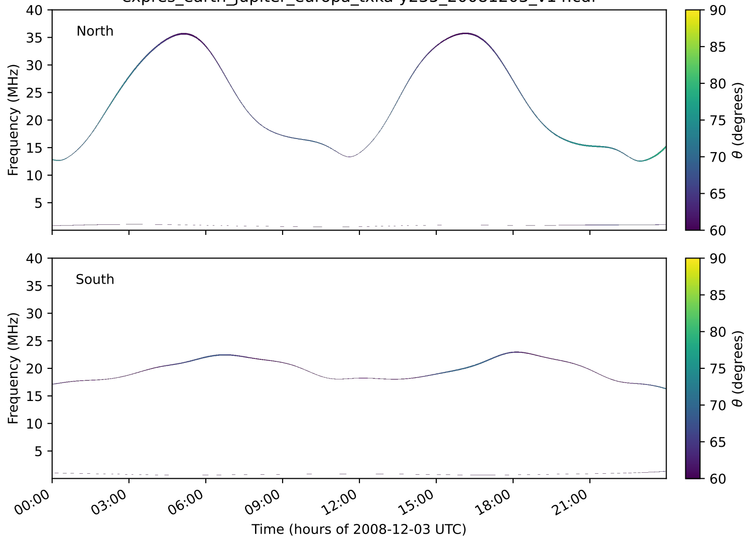
expres_earth_jupiter_europa_txka-y235_20081203_v14.cdf
