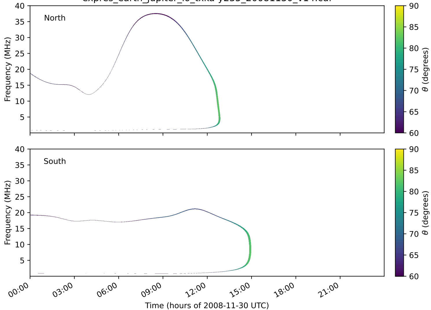
expres_earth_jupiter_io_txka-y235_20081130_v14.cdf
