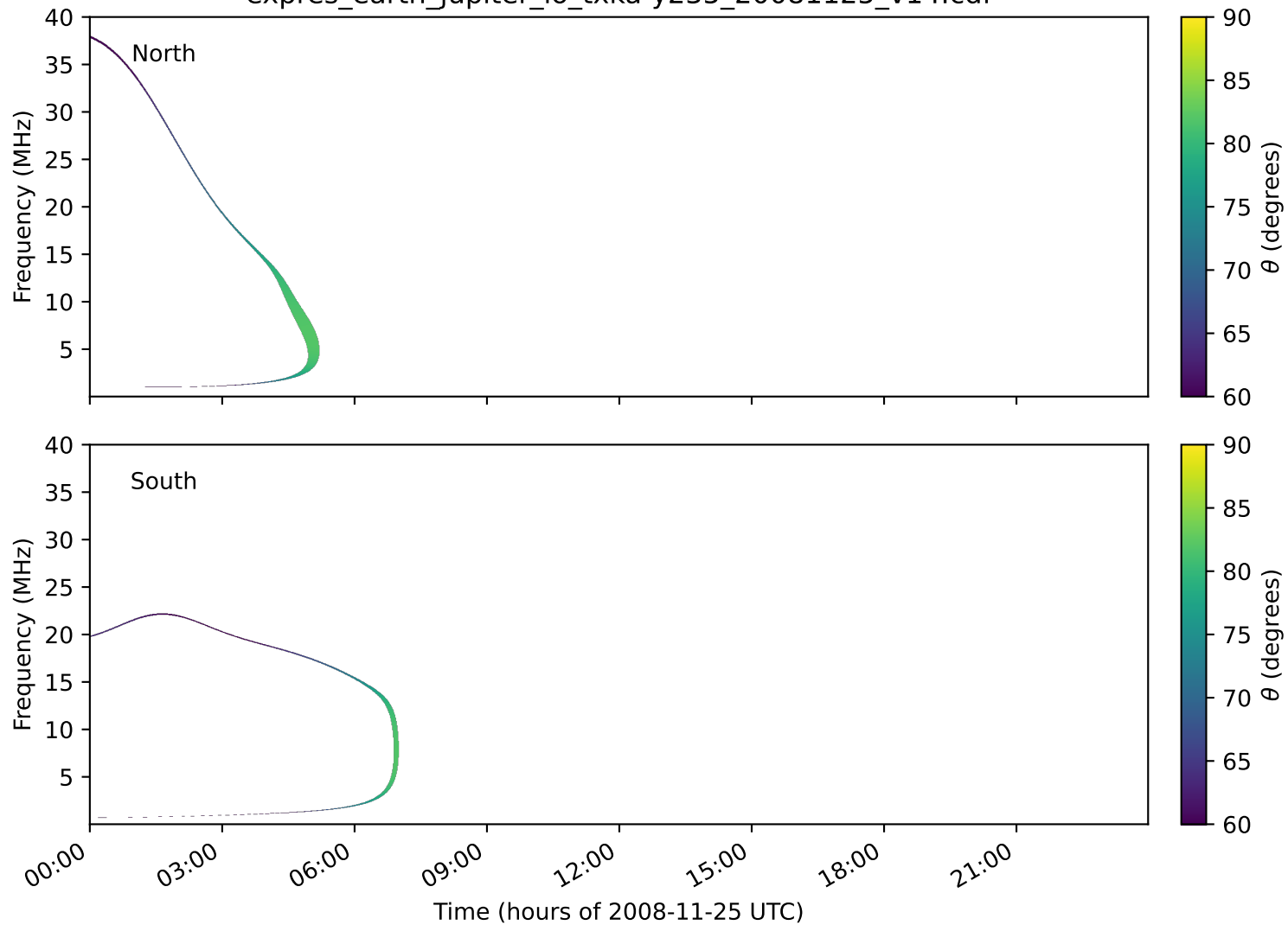
expres_earth_jupiter_io_txka-y235_20081125_v14.cdf
