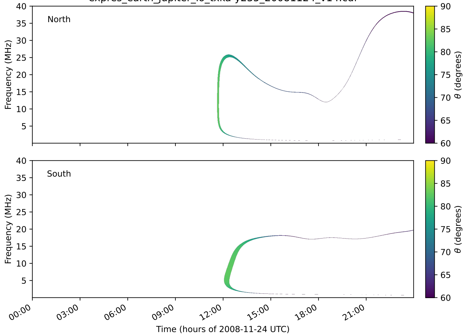
expres_earth_jupiter_io_txka-y235_20081124_v14.cdf
