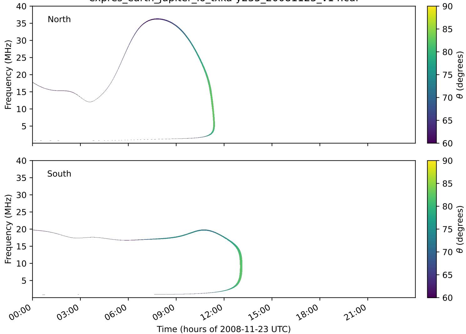
expres_earth_jupiter_io_txka-y235_20081123_v14.cdf
