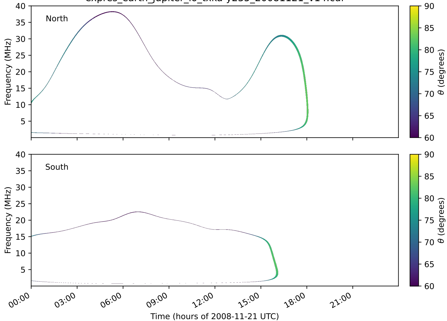
expres_earth_jupiter_io_txka-y235_20081121_v14.cdf
