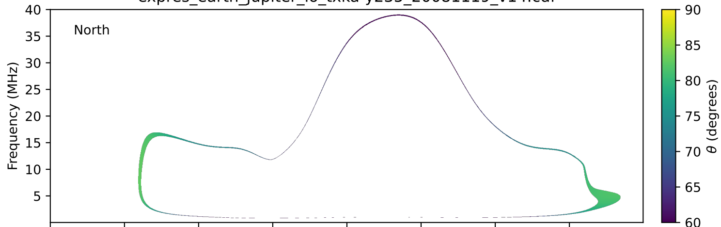
expres_earth_jupiter_io_txka-y235_20081119_v14.cdf
