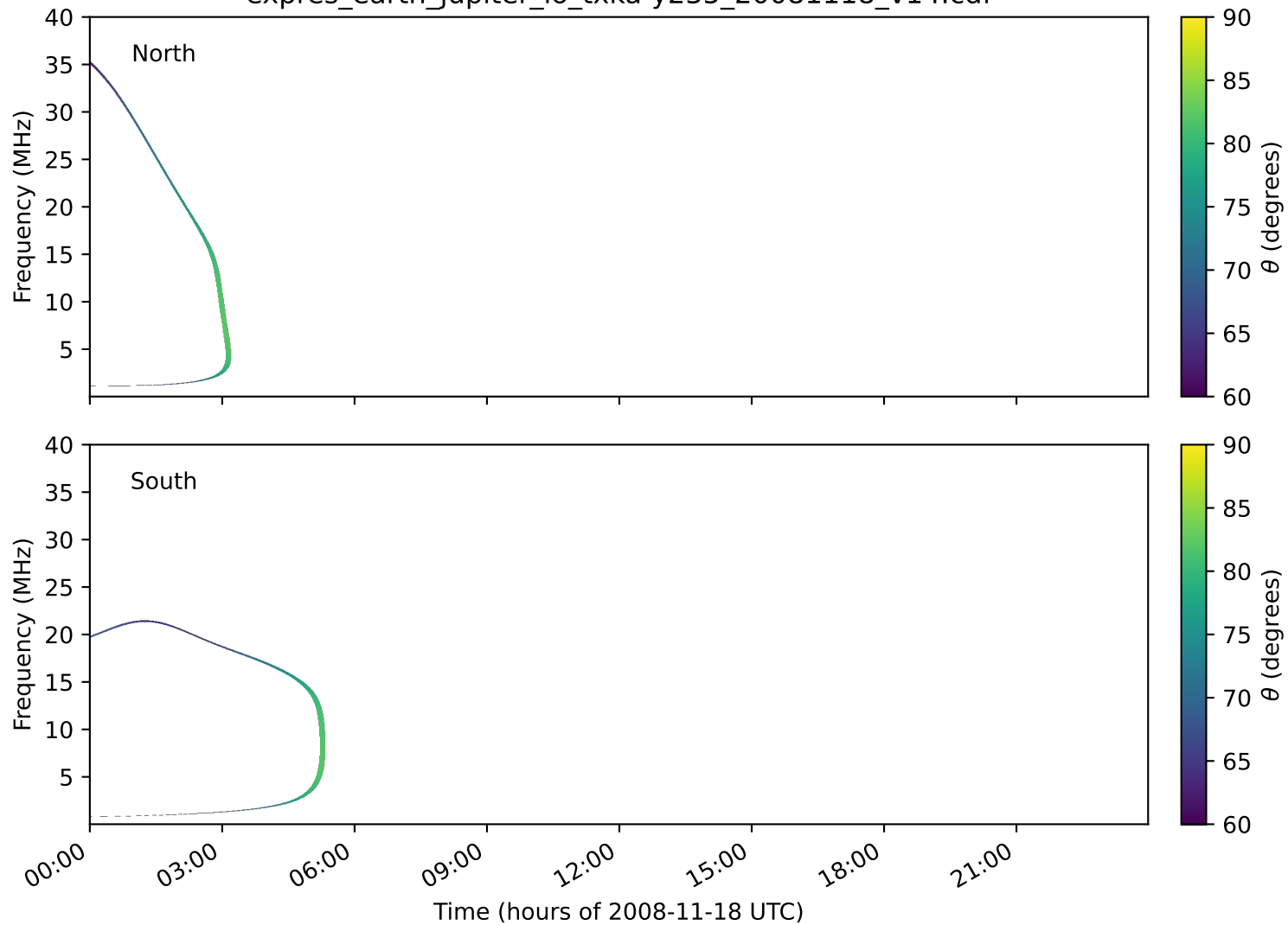
expres_earth_jupiter_io_txka-y235_20081118_v14.cdf
