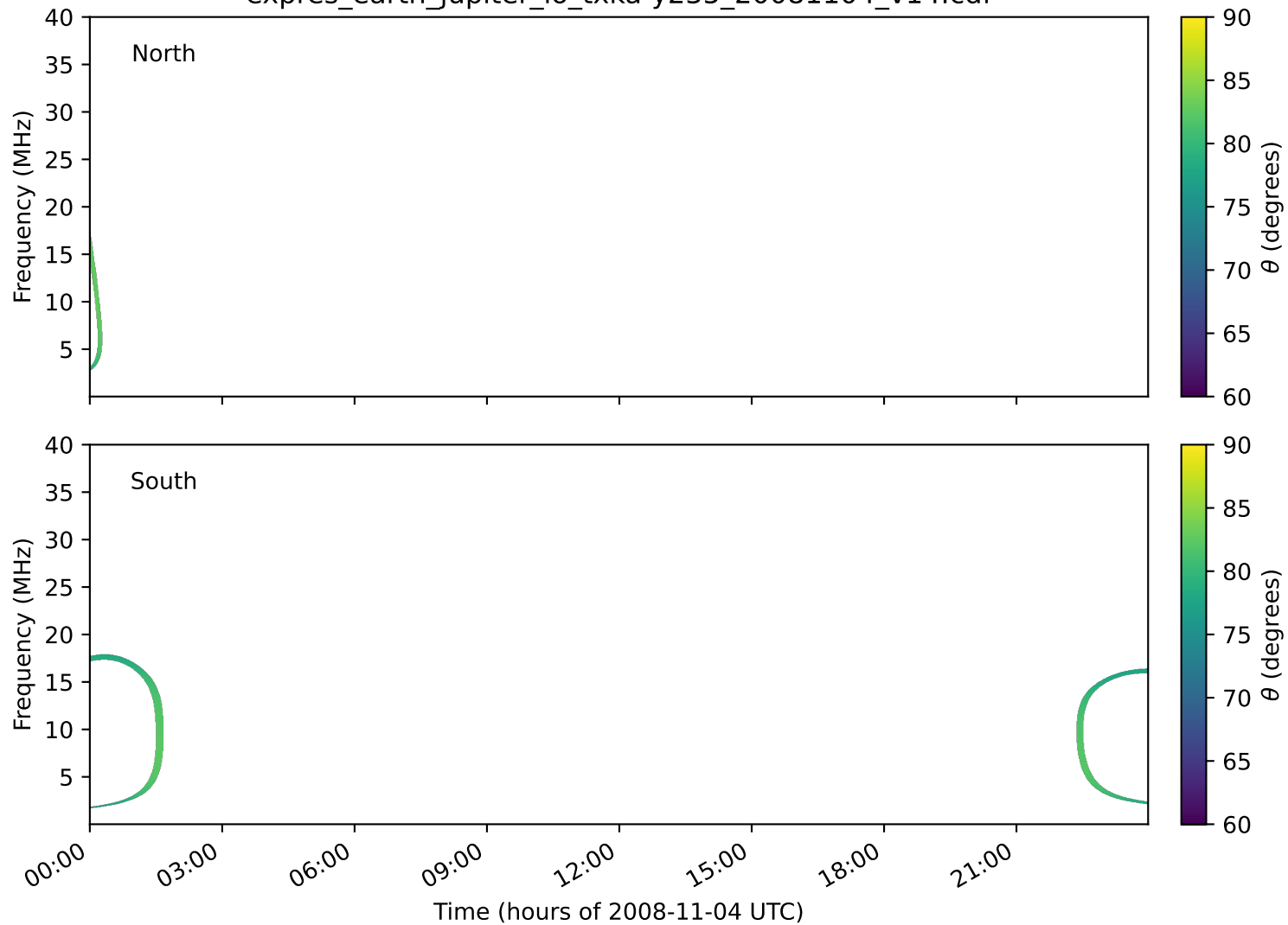
expres_earth_jupiter_io_txka-y235_20081104_v14.cdf
