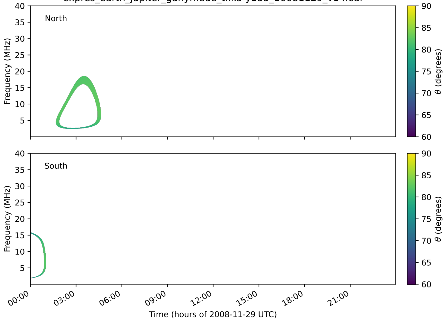
expres_earth_jupiter_ganymede_txka-y235_20081129_v14.cdf
