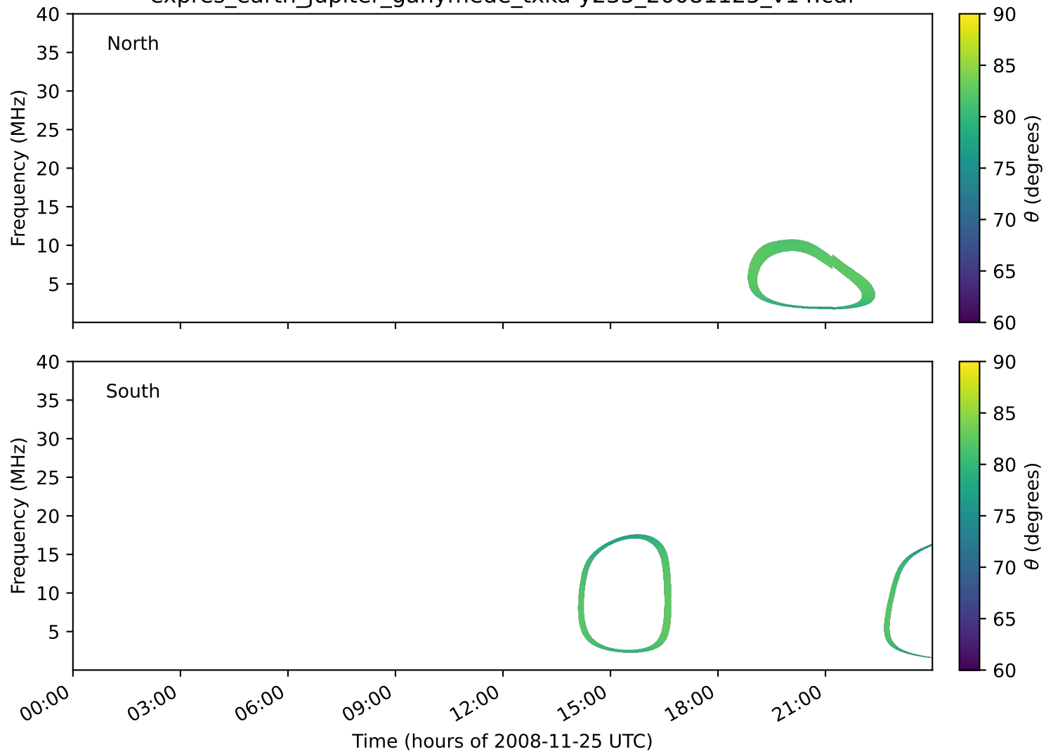
expres_earth_jupiter_ganymede_txka-y235_20081125_v14.cdf
