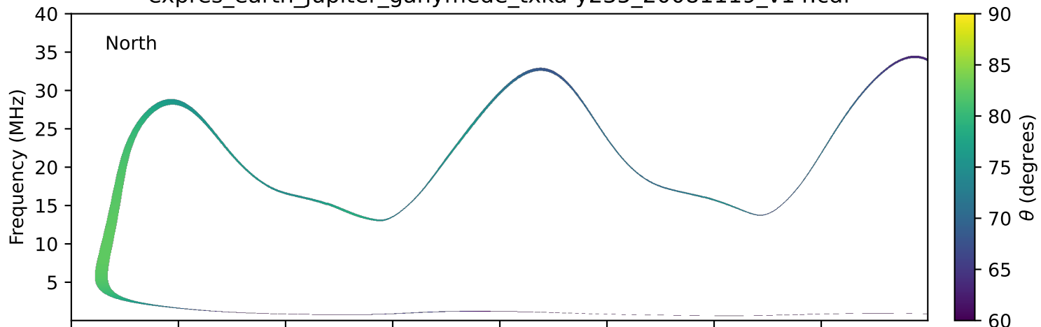
expres_earth_jupiter_ganymede_txka-y235_20081119_v14.cdf
