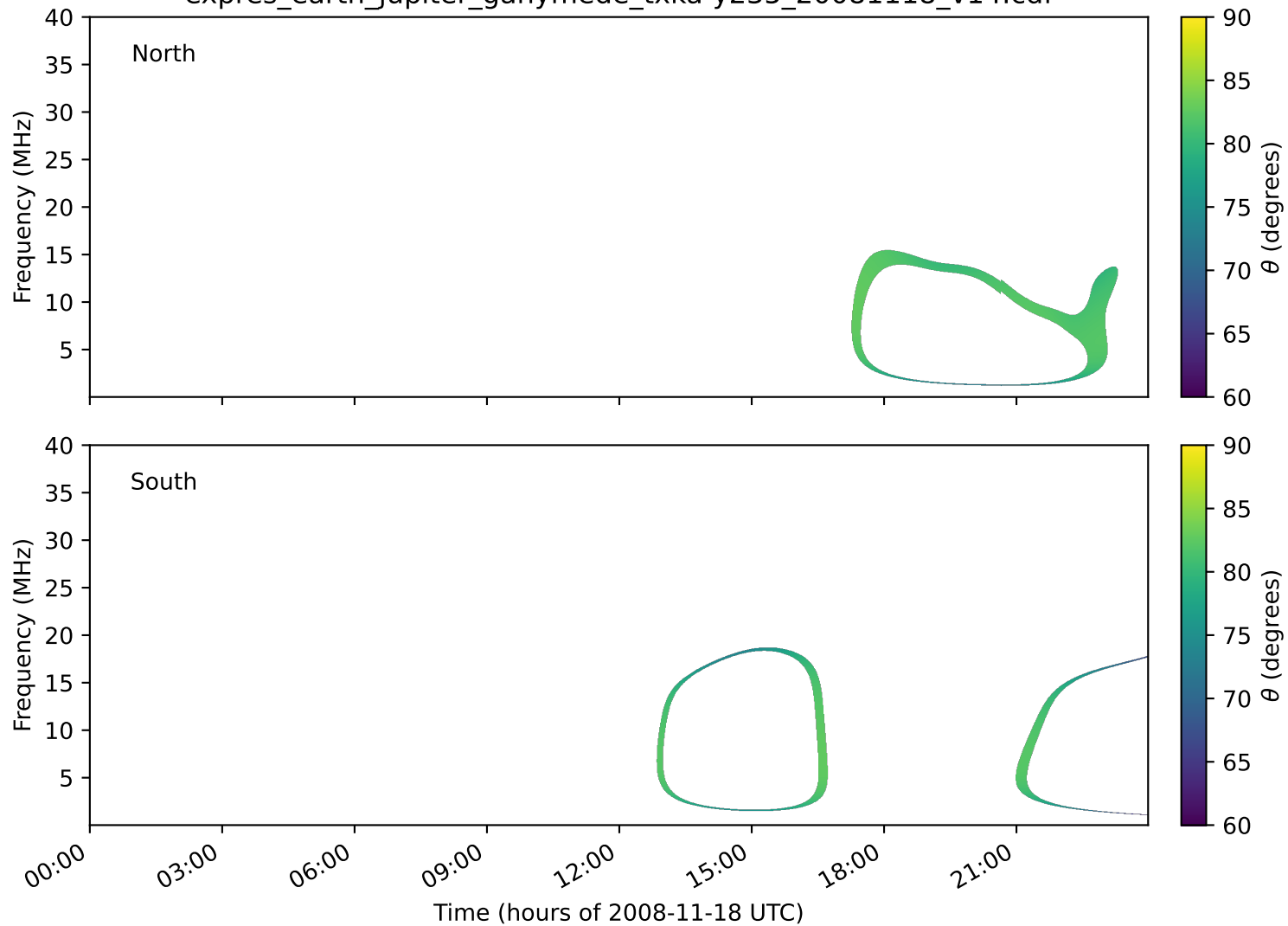
expres_earth_jupiter_ganymede_txka-y235_20081118_v14.cdf
