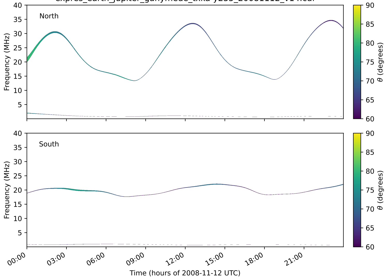
expres_earth_jupiter_ganymede_txka-y235_20081112_v14.cdf
