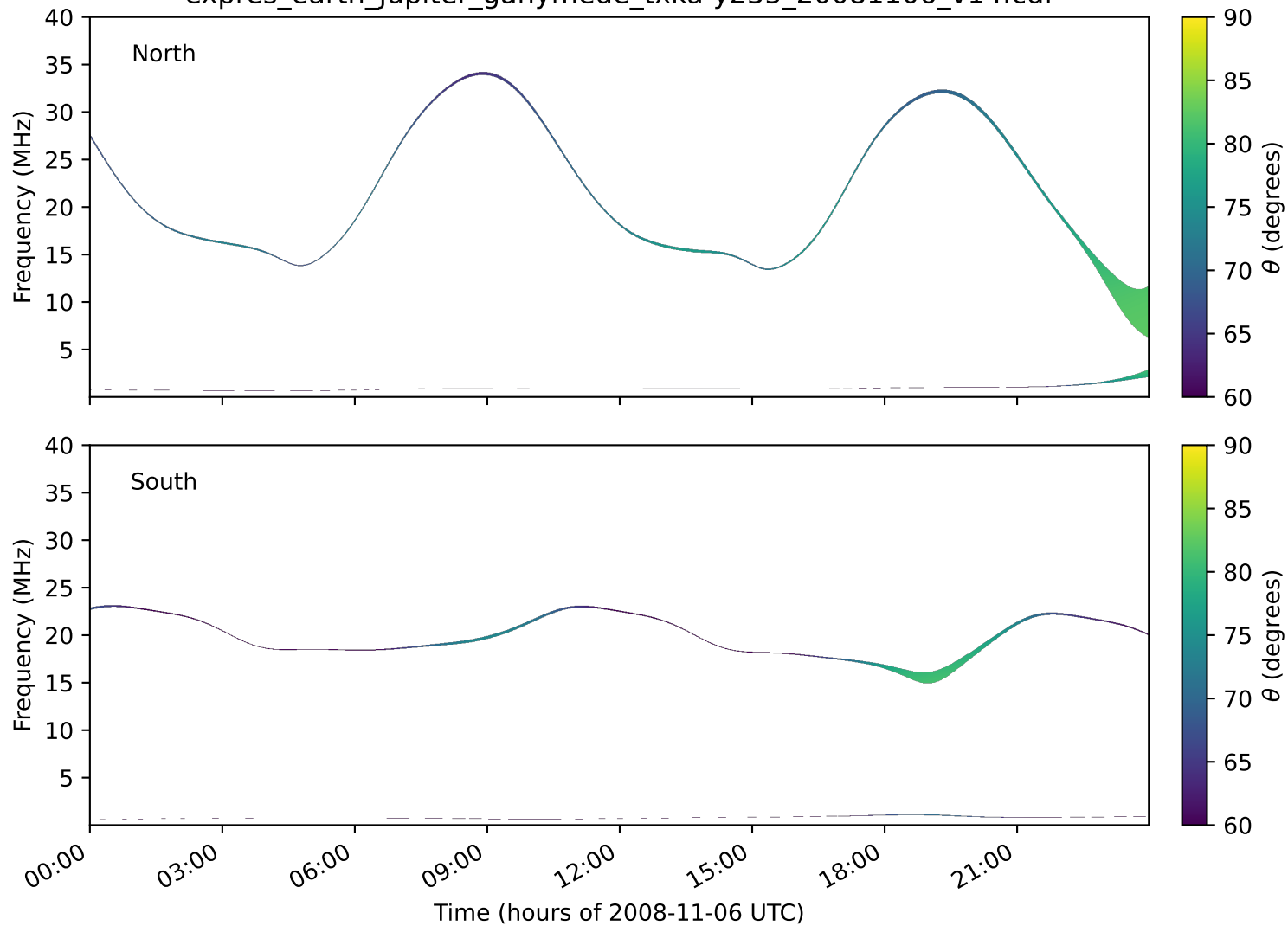
expres_earth_jupiter_ganymede_txka-y235_20081106_v14.cdf
