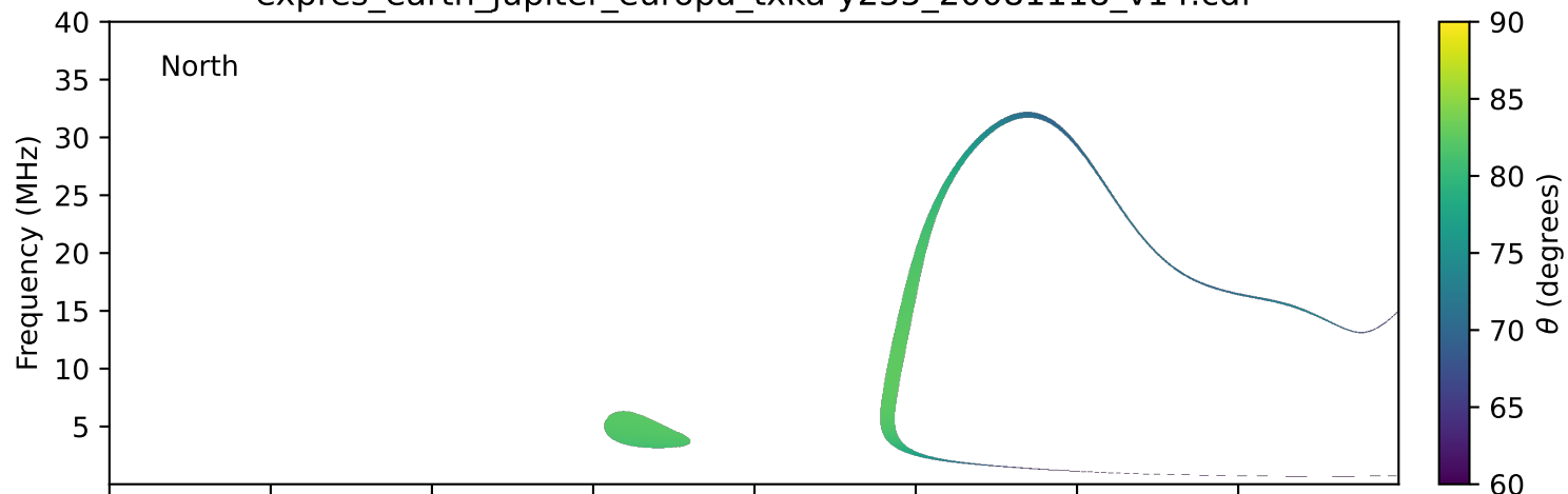
expres_earth_jupiter_europa_txka-y235_20081118_v14.cdf
