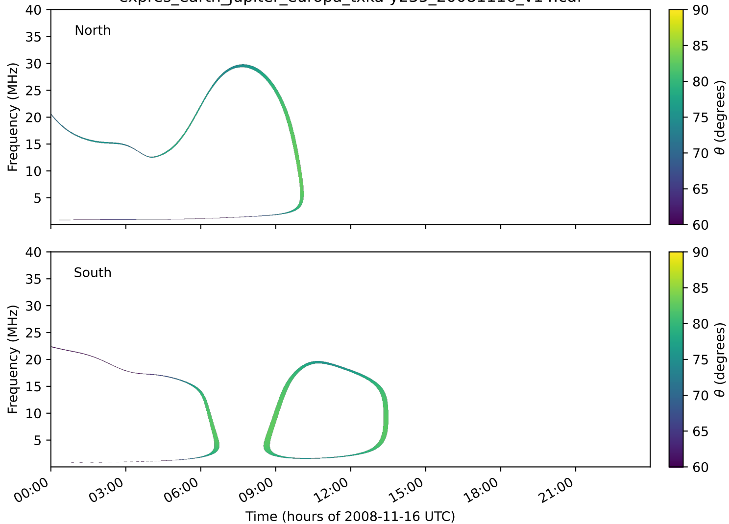
expres_earth_jupiter_europa_txka-y235_20081116_v14.cdf
