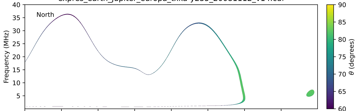
expres_earth_jupiter_europa_txka-y235_20081112_v14.cdf
