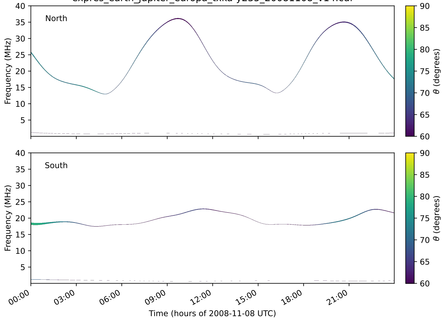
expres_earth_jupiter_europa_txka-y235_20081108_v14.cdf
