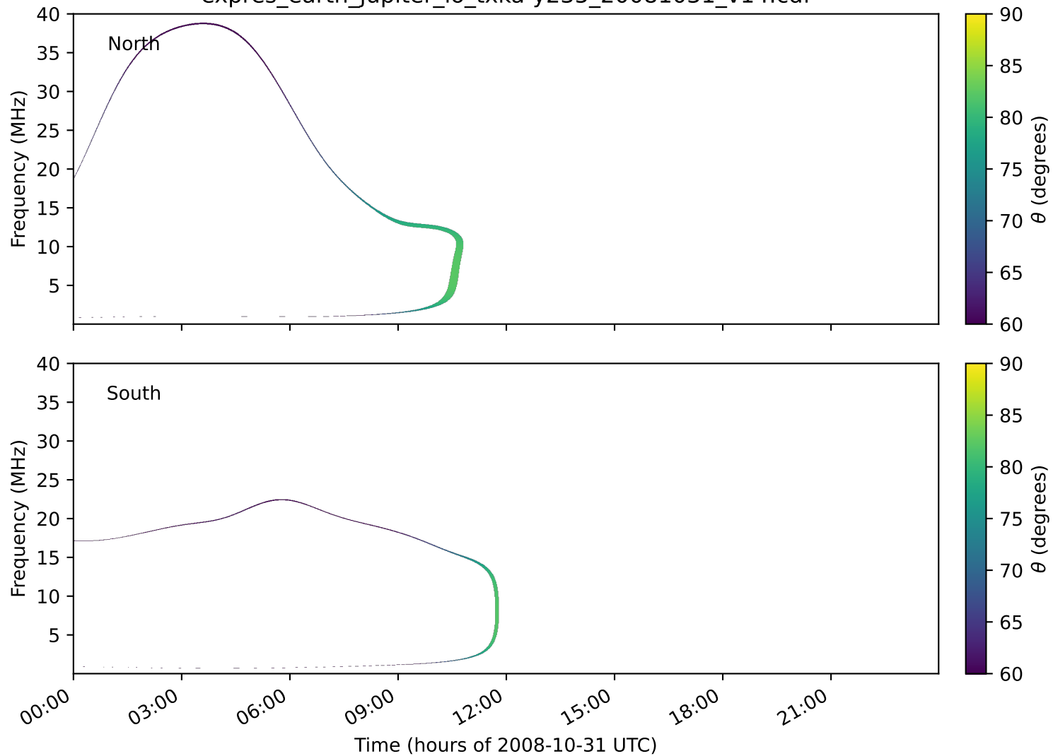
expres_earth_jupiter_io_txka-y235_20081031_v14.cdf
