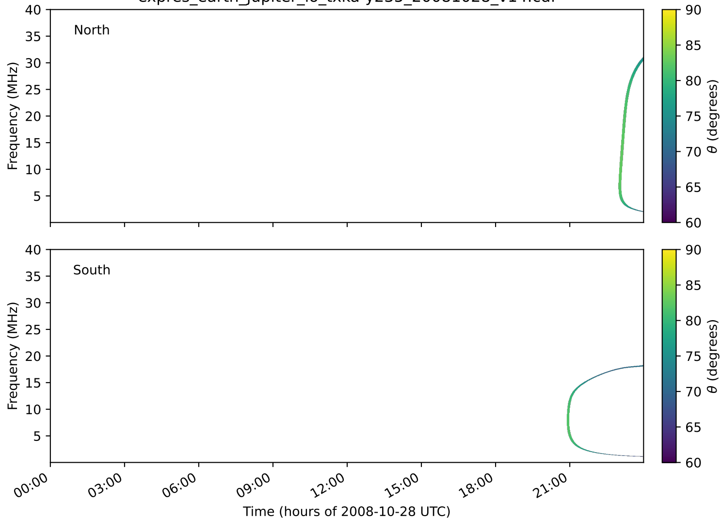
expres_earth_jupiter_io_txka-y235_20081028_v14.cdf
