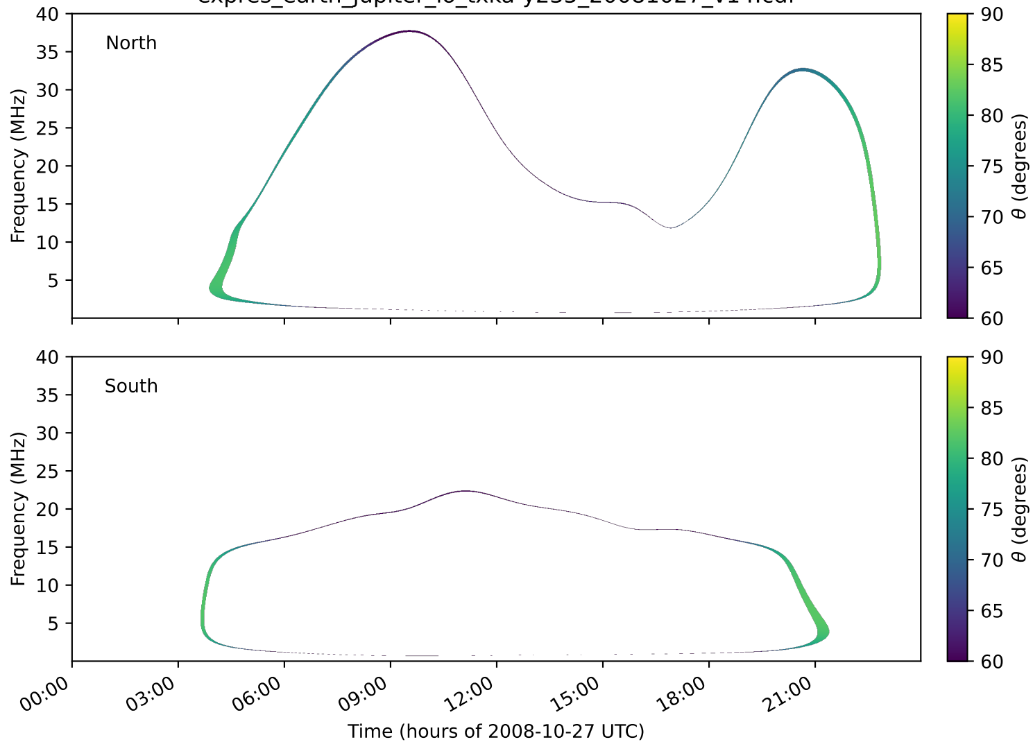
expres_earth_jupiter_io_txka-y235_20081027_v14.cdf
