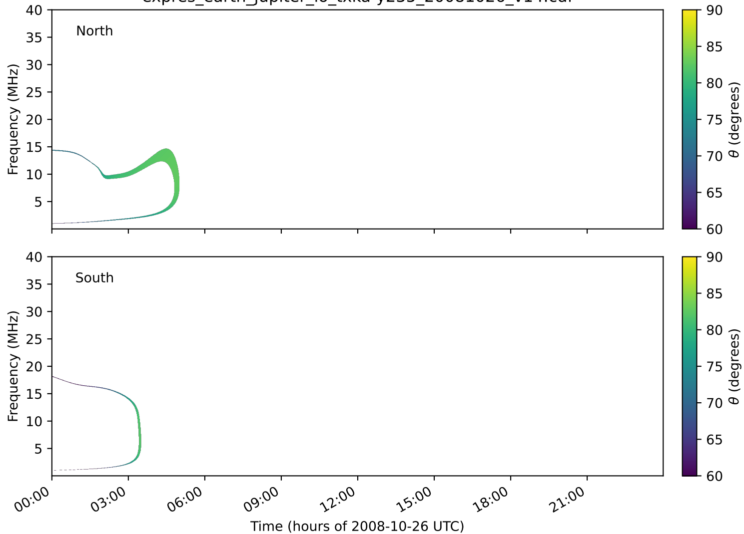
expres_earth_jupiter_io_txka-y235_20081026_v14.cdf
