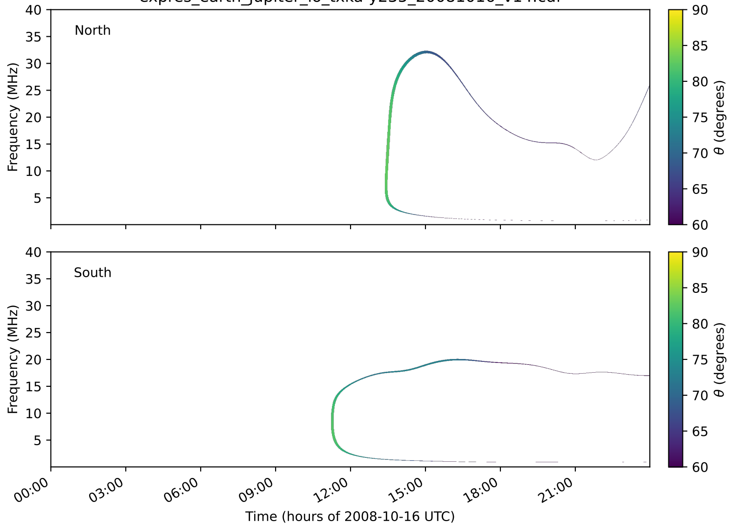
expres_earth_jupiter_io_txka-y235_20081016_v14.cdf
