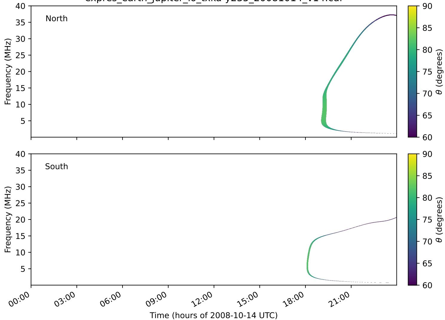
expres_earth_jupiter_io_txka-y235_20081014_v14.cdf
