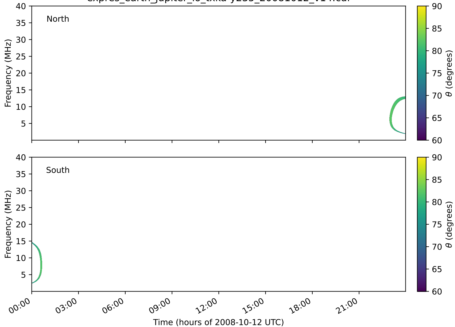
expres_earth_jupiter_io_txka-y235_20081012_v14.cdf
