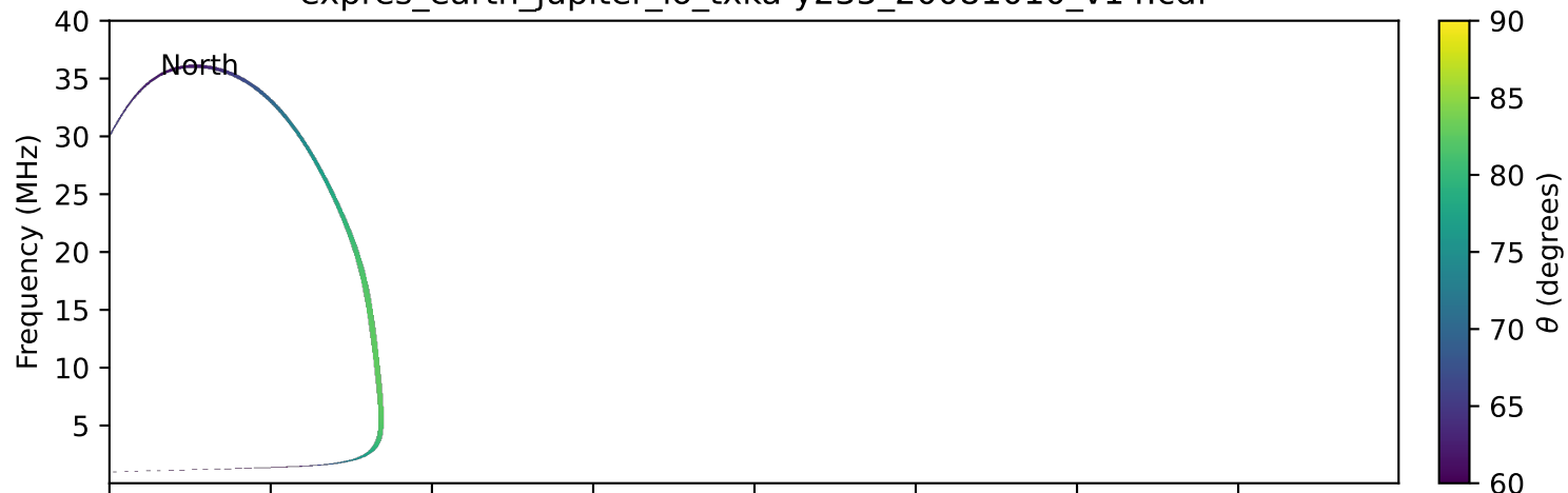
expres_earth_jupiter_io_txka-y235_20081010_v14.cdf
