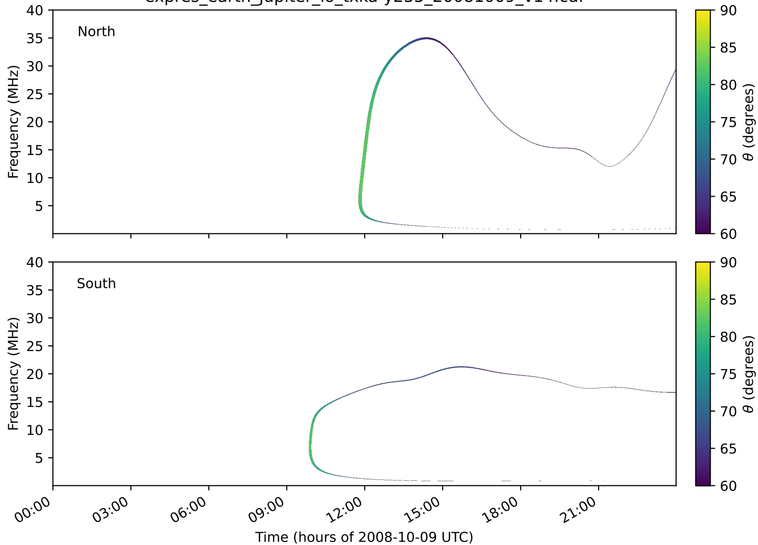
expres_earth_jupiter_io_txka-y235_20081009_v14.cdf
