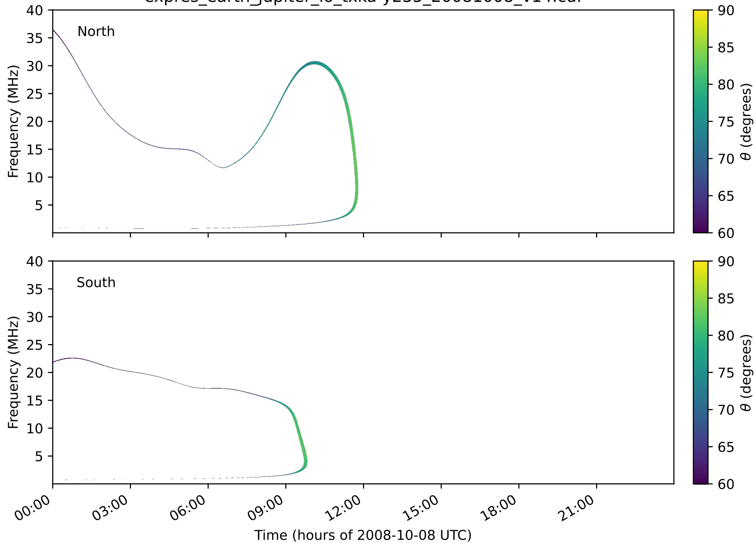
expres_earth_jupiter_io_txka-y235_20081008_v14.cdf
